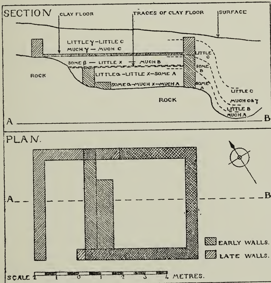
Fig. 7. Plan and section to illustrate graphic publication.
